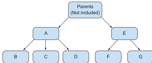
Figure 7.1 Graph of the family for nested list comprehensions
