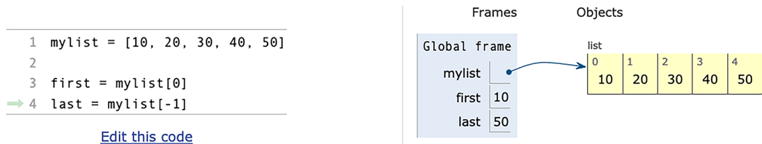
Figure 3.1 Individual elements (from the Python Tutor)
