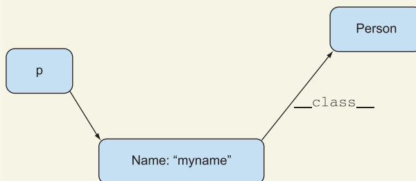
Figure 9.6 Finally, __init__ exits, and the object in __new__ is returned to the caller.
