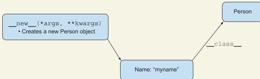
Figure 9.5 __init__ adds attributes to the object.
