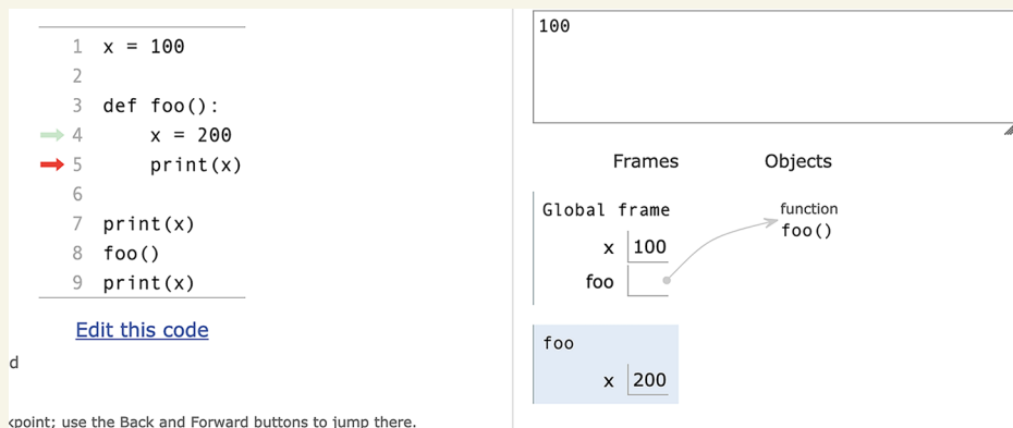
Figure 6.2 Inner vs. outer x
