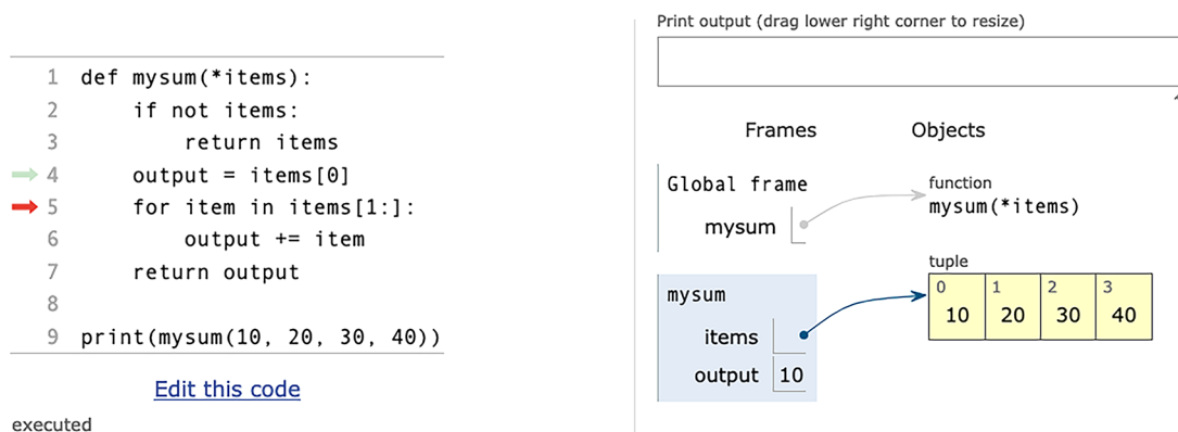
Figure 3.6 After assigning the first element to output (from the Python Tutor)
