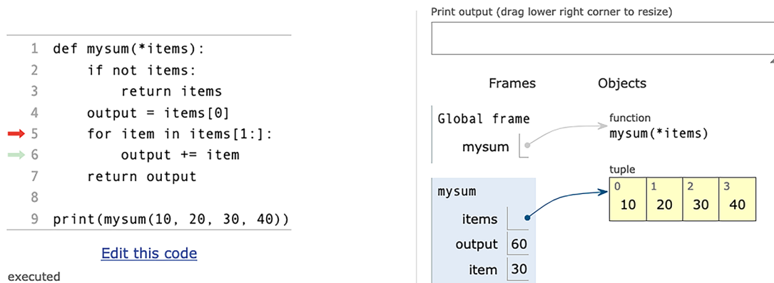
Figure 3.7 After adding elements to output (from the Python Tutor)
