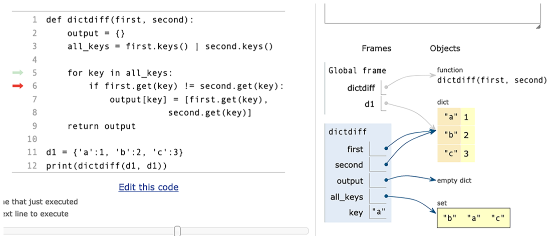
Figure 4.5 Iterating over the keys of d1
